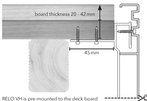
RELO VH holder
